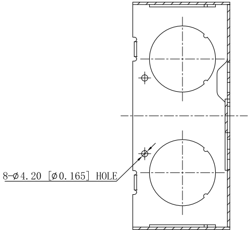
CUTAWAY VIEW A-A
