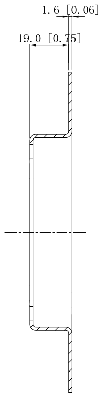
CUTAWAY VIEW A-A
