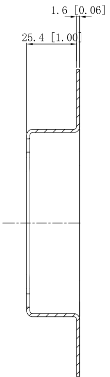
CUTAWAY VIEW A-A
