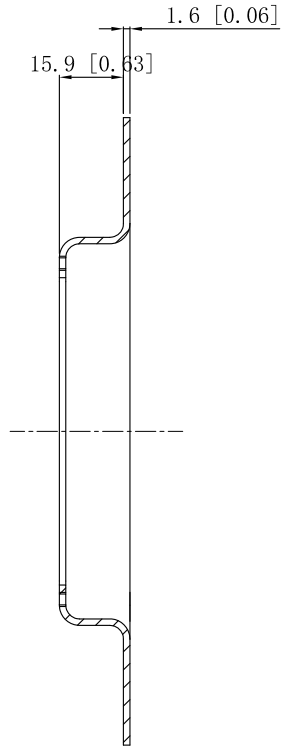
CUTAWAY VIEW A-A
