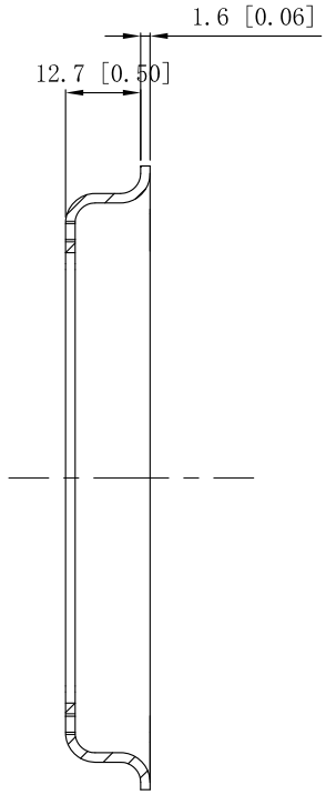
CUTAWAY VIEW A-A
