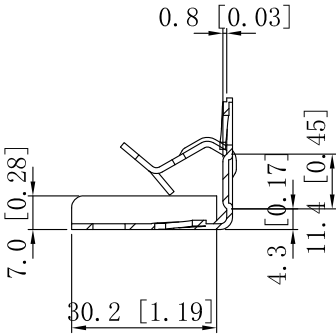
CUTAWAY VIEW A-A
