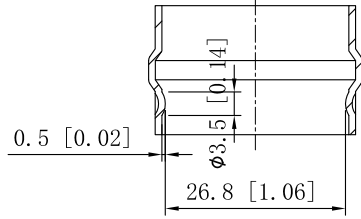
CUTAWAY VIEW C-C
