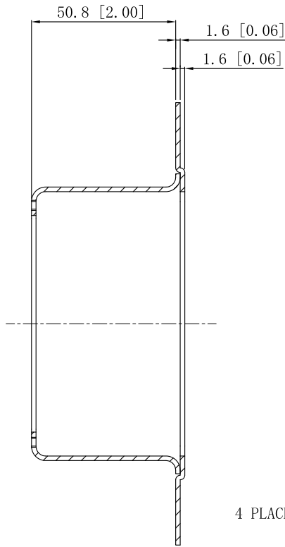
CUTAWAY VIEW A-A
