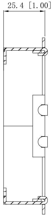
CUTAWAY VIEW A-A
