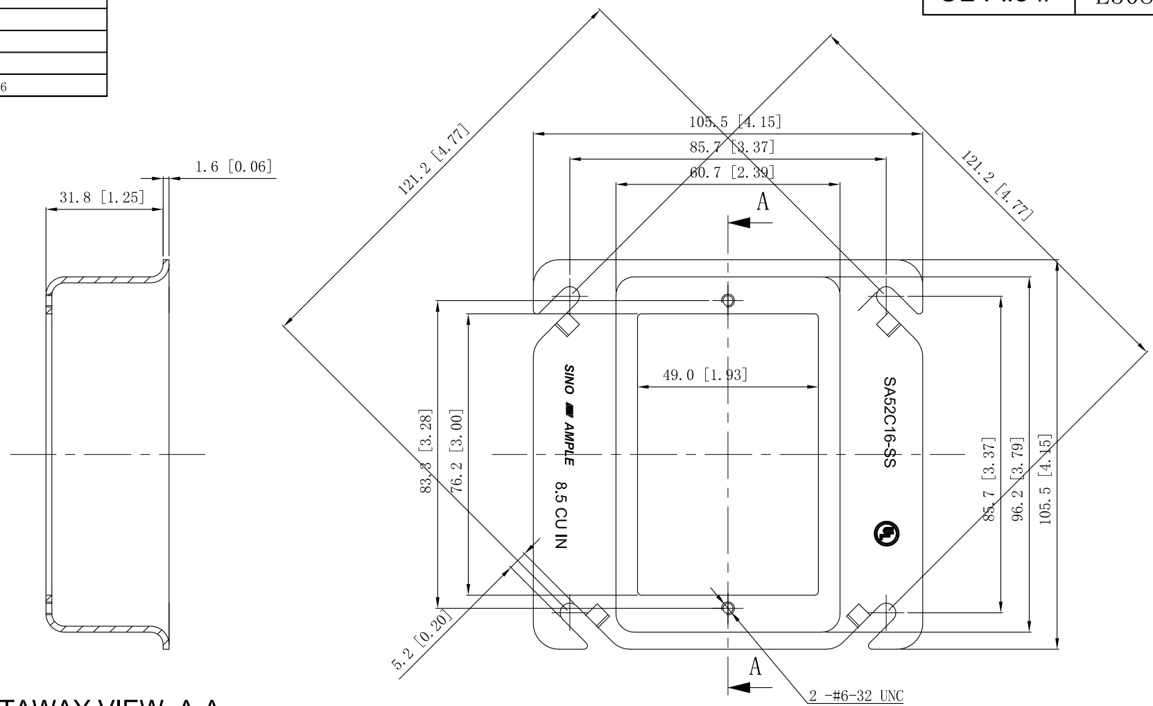
CUTAWAY VIEW A-A
