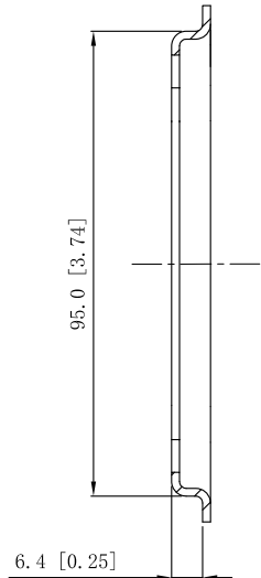
CUTAWAY VIEW B-B
