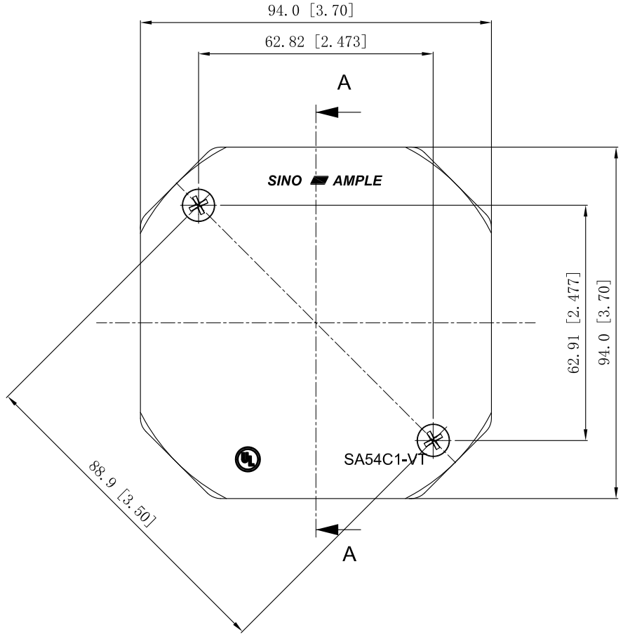
#8-32 UNC, x 2
