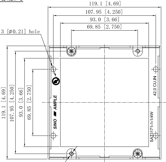
WELDING STYLE DETAIL VIEW D
